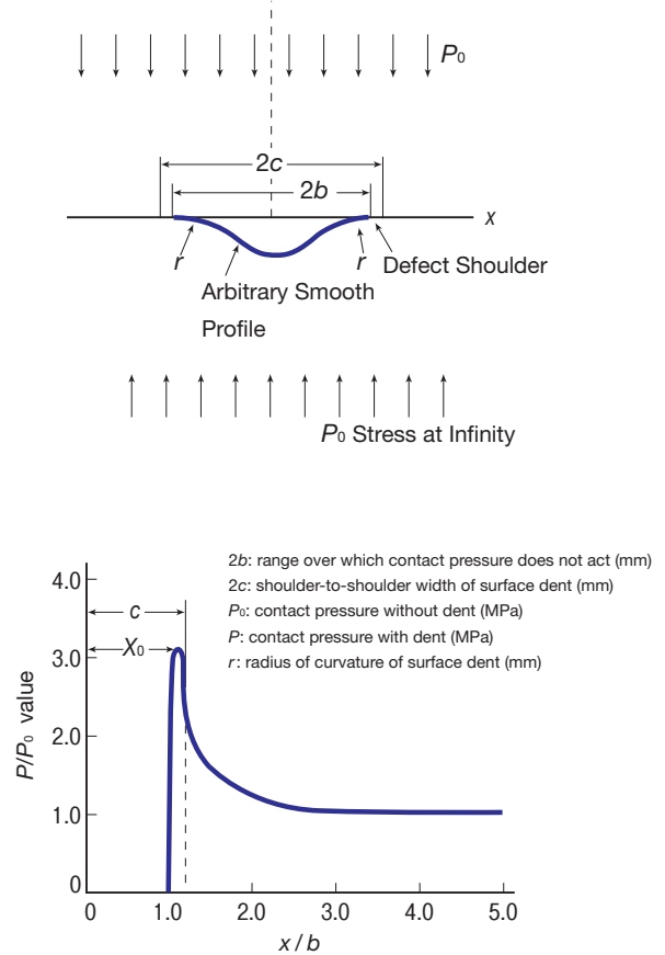
Fig. 2 Concentration of stress around a surface dent
