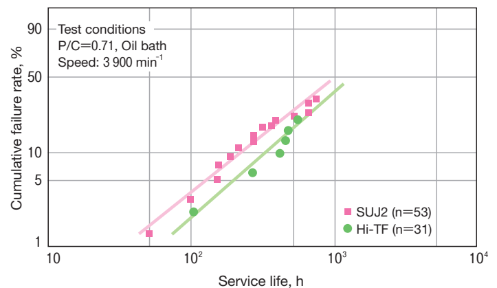
Fig. 8 Service life tests of 6206 bearings under clean lubrication
