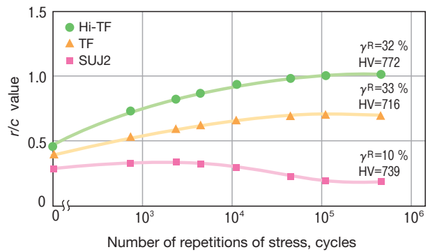
Fig. 5 Change of r/c value under repeated stress
