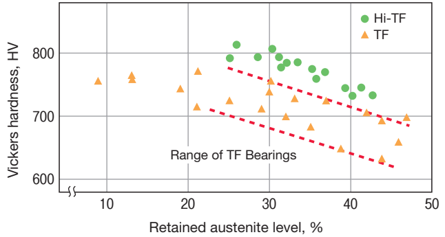
Fig. 4 Relationship of material hardness and retained austenite level
