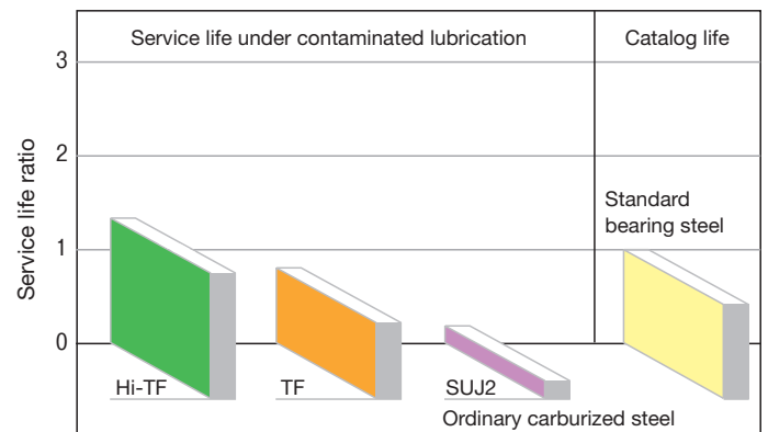
Fig. 7 Comparison of service life under contaminated lubrication
