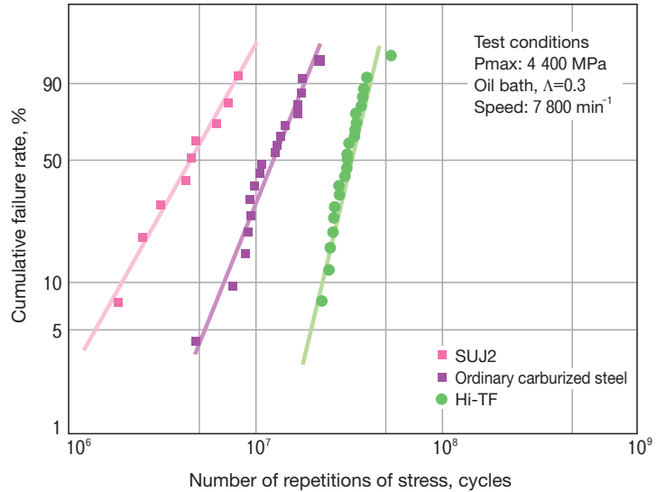
Fig. 9 Service life tests with boundary lubrication conditions
