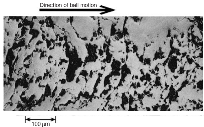
Fig. 10 Peeling damage
