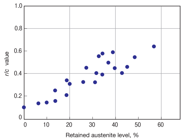
Fig. 3 Relationship of r/c value to retained austenite level
