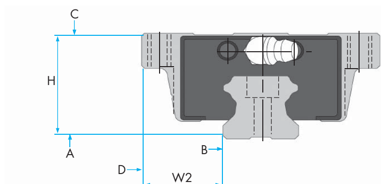
Figure 2. Block measurement
