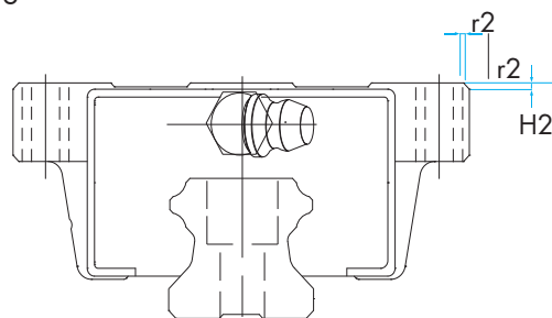
Assembly of block datum plane
