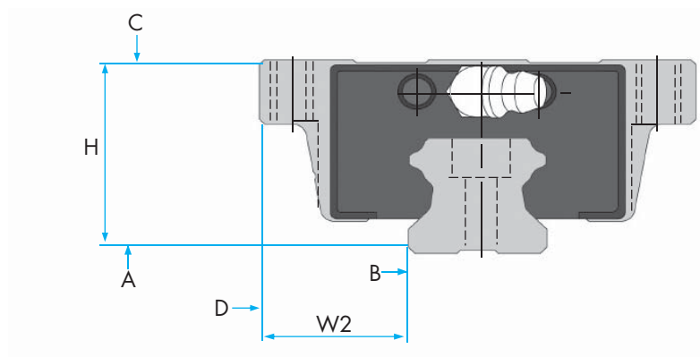
Figure 3. Block measurement
