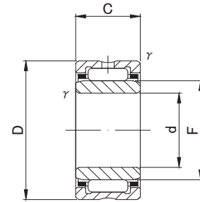
NA49,NA59,NA69( d \leq 30 ),NKI
