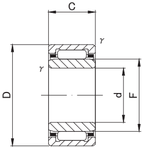
NKI(d ≤ 8)
