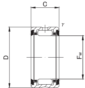
RNA49UU, RNA69UU ( F_w \leq 35 )
