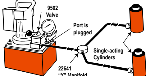
Single-acting cylinder or cylinders in the circuit, controlled by a pump-mounted valve.
