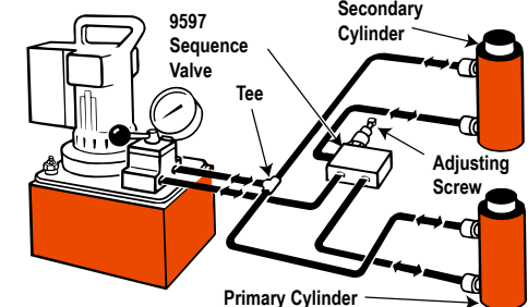
Double-acting cylinder with a sequence valve which controls the primary and secondary cylinder circuits.
