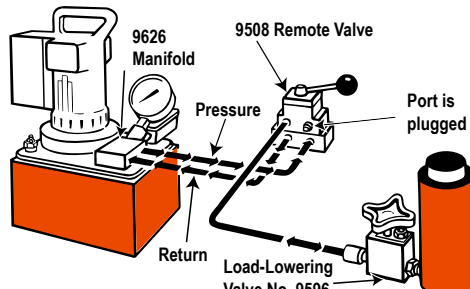
Single-acting cylinder controlled by a remote-mounted valve.
