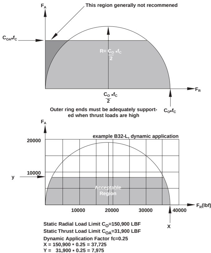
Figure 13: Radial Bearings
