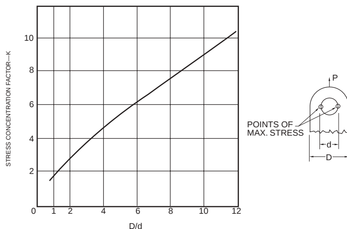
Figure 16: Stress Concentration Factor
