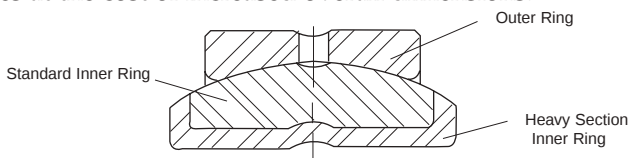
Figure 5: Standard vs. Heavy Section Inner Ring
