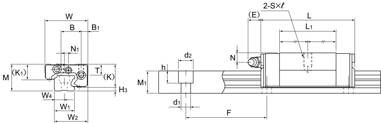
Model GSR15T/V
