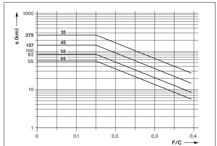
Fig. 3: Relubrication interval
